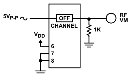
Figure 20. Feedthrough (All Types)
