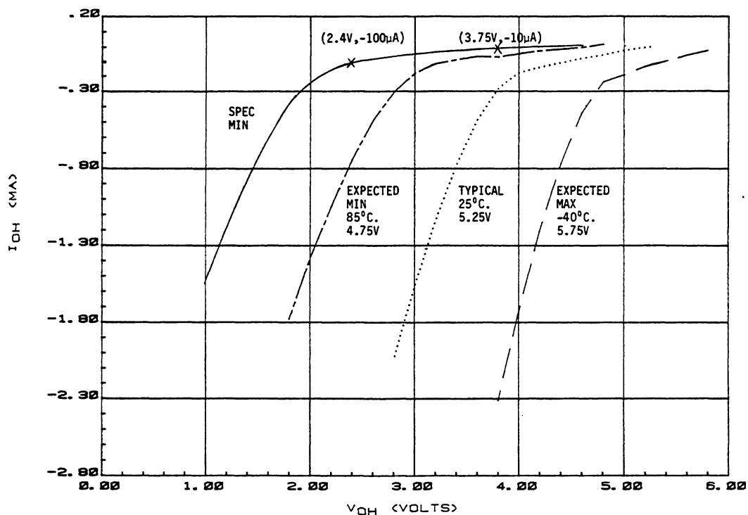
Figure 11-4. Port A V_{OH} vs I_{OH} (With CMOS Pull-Ups)
