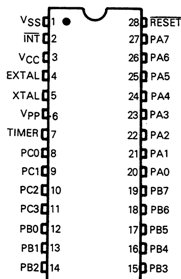
MC68705P3
