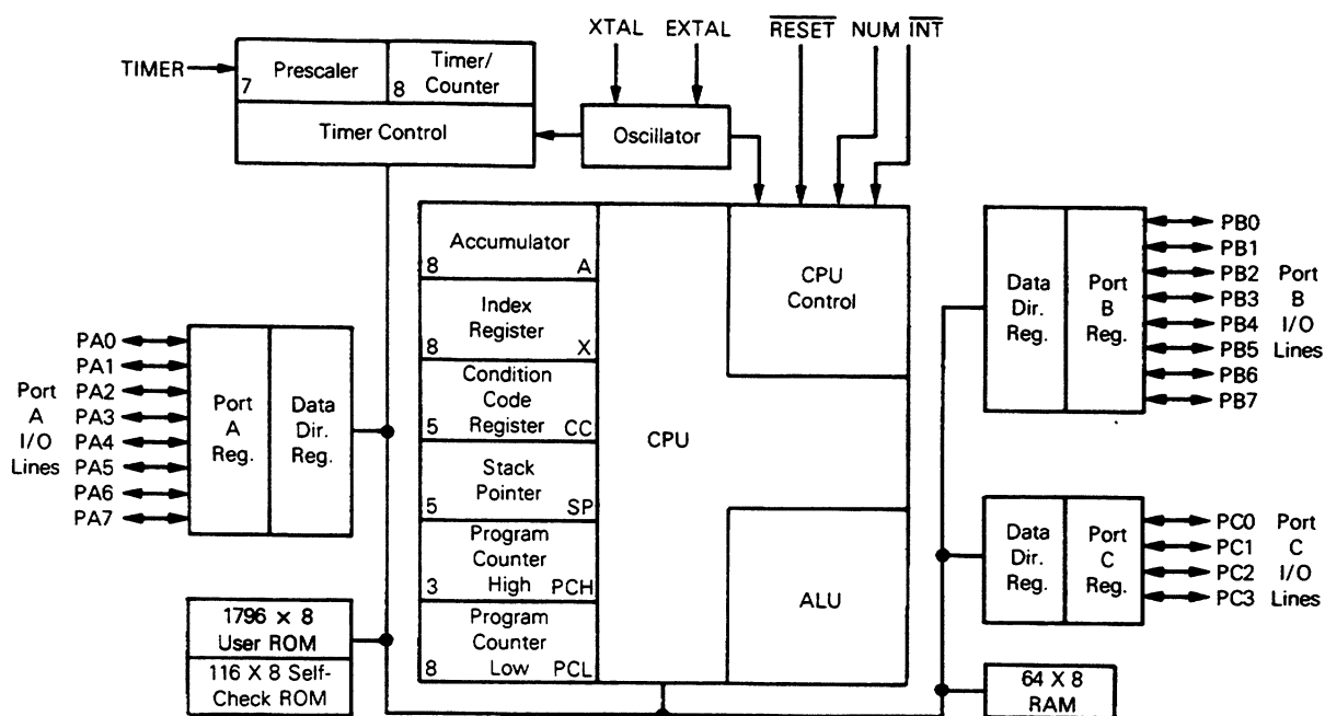
Figure 1-3. MC6805P6 Block Diagram
