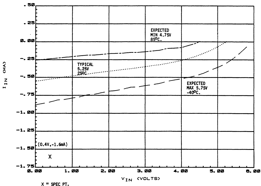
Figure 11-11. EXTAL V_{in} vs I_{in}
