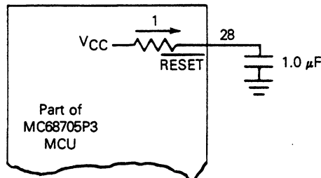
Figure 7-3. Power-Up \overline{\text{RESET}} Delay Circuit
