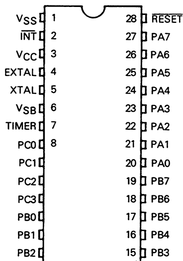
MC6805P4
