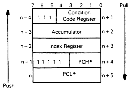
Figure 3-5. Interrupt Stacking Order
