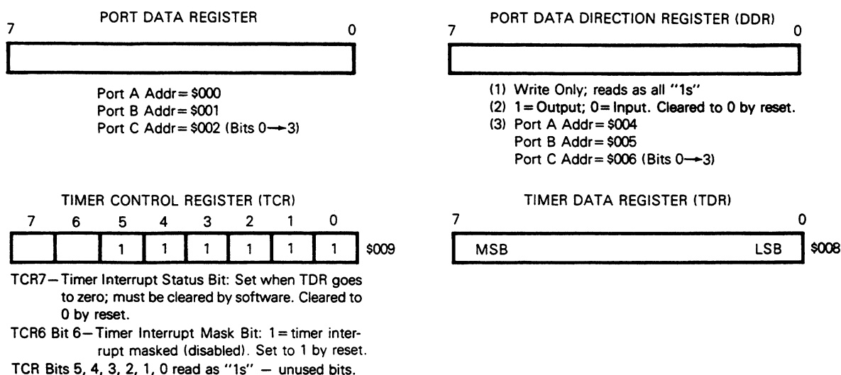
Figure 8-2. MCU Register Configuration for MC6805P2/P4/P6
