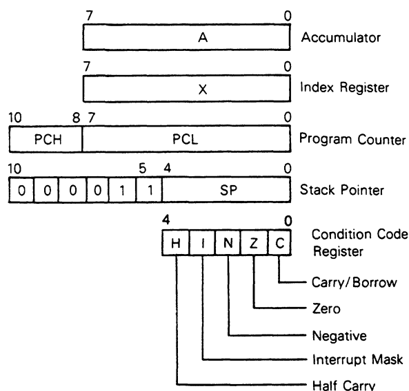
Figure 4-1. Programming Model
