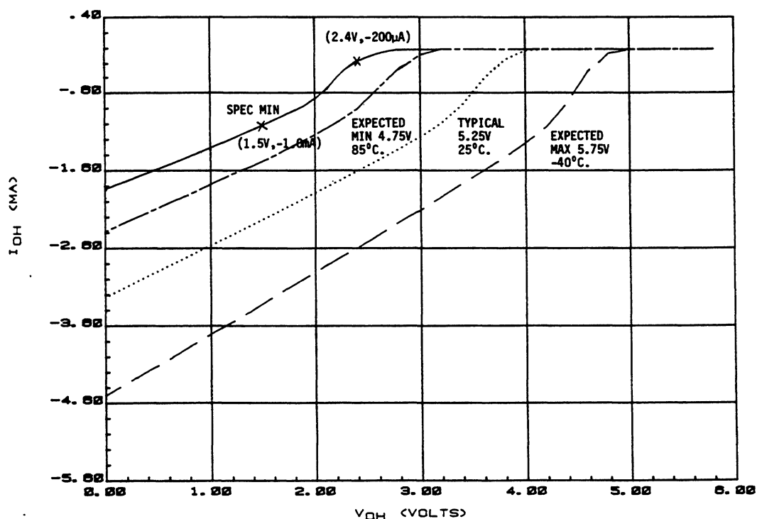
Figure 11-6. Port B V_{OH} vs I_{OH}
