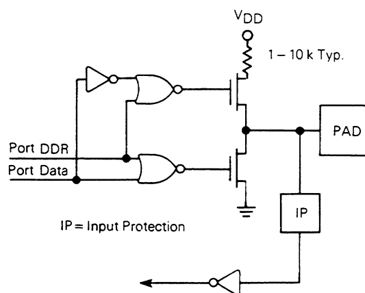
Figure 11-16. Port B Logic Diagram
